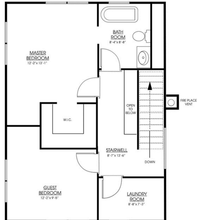
UPPER FLOOR PLAN - 660 SQ FT Equinox
