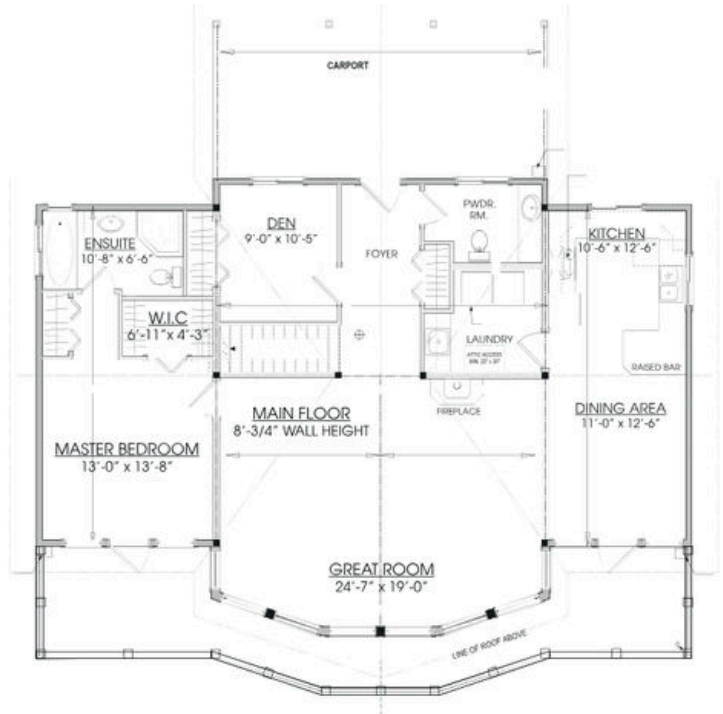
MAIN FLOOR PLAN - 1504 SQ FT Harbour Side II
