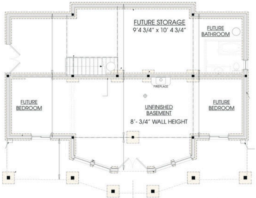
LOWER LEVEL FLOOR PLAN - 1504 SQ FT Harbour Side II
